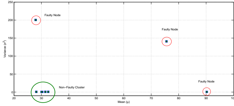
Fig. 3. Scatter plot of dataset statistics -Data Source [Lim and Bleakley 2010]
