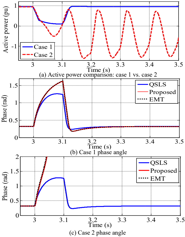
Fig. 5. Result when V_g steps down to 0.363 pu at 3 s and recovered at 3.1 s.
