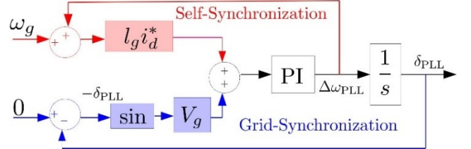
Fig. 3. Quasi-static large-signal model of the PLL [6]
