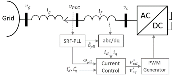
Fig. 1. Grid-Feeding Converter system structure
