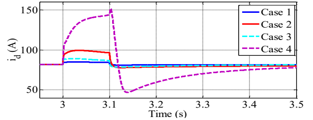
Fig. 6. d-axis current transient result when V_g steps down to 0.569 pu and recovered at 3.1 s.
