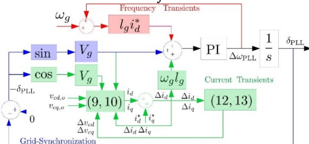
Fig. 4. Advanced synchronization stability assessment
