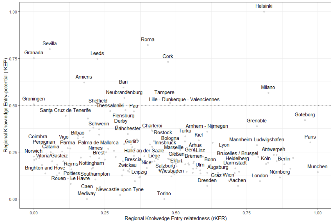
Figure 5. Position of EU15 Metropolitan regions in in rKER and rKEP (2011-2015)
