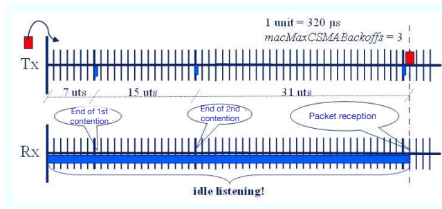
Fig. 4. Receiver idle listening of the CSMA period in 802.15.4
