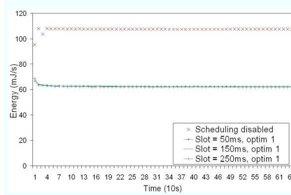
Fig. 9. Optimization 1: energy consumption results at transmitter side
