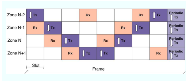
Fig. 2. The table of scheduling with periodic local broadcast
