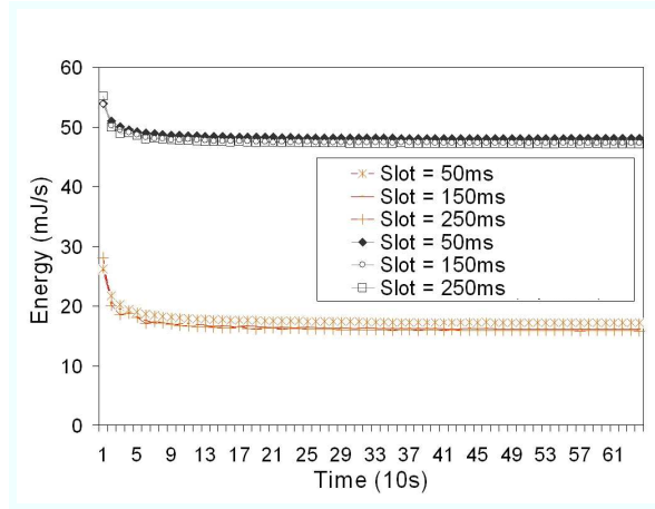
Fig. 12. Optimization 3 energy consumption results
