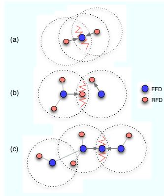
Fig. 1. (a) HTP in single-hop 802.15.4, (b) HTP with nearby independent star networks, and (c) HTP with aggregated star networks in multi-hop deployments
