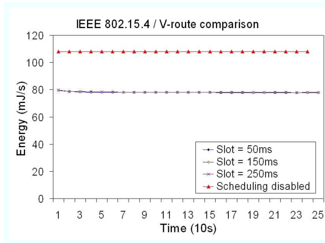
Fig. 8. Comparison between the energy consumption of a plain multihop-enabled 802.15.4 and 802.15.4 enhanced with V-route.
