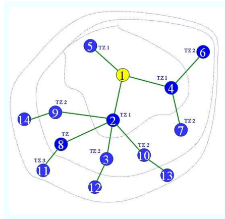
Fig. 3. The initial timezone setup by flooding and different path generation
