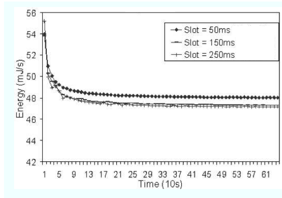
Fig. 11. Optimization 2 energy consumption results
