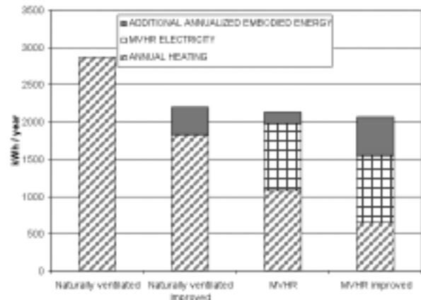
Fig 6: Annual primary energy use for heating, MVHR electricity, and annualized EE, in kWh.
