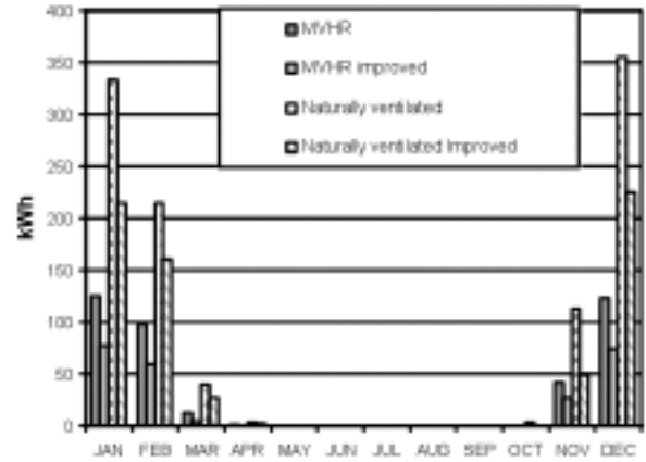
Figure 5: Monthly heating demand for the four different options
