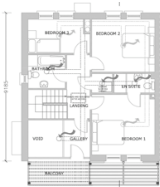
Figure 3: Prototype passive house first floor plan. [7]
