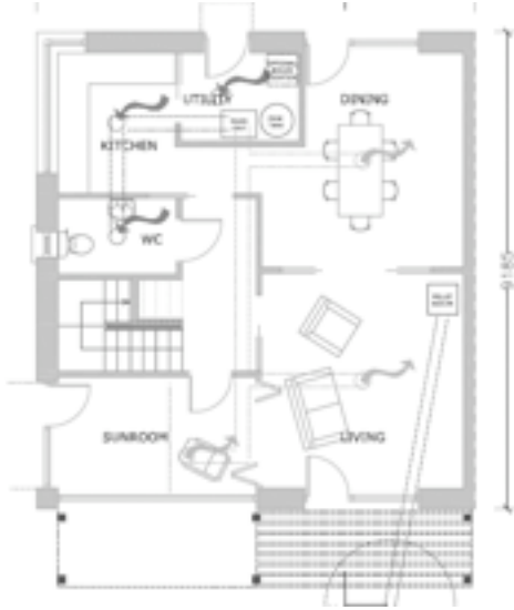
Figure 2: Prototype passive house ground floor plan. [7]
