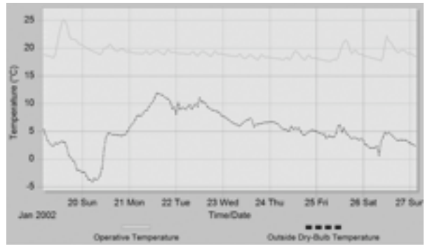
Fig 7: Outside and living room temperatures on a typical winter week, for the ‘free running’ natural ventilation improved option.
