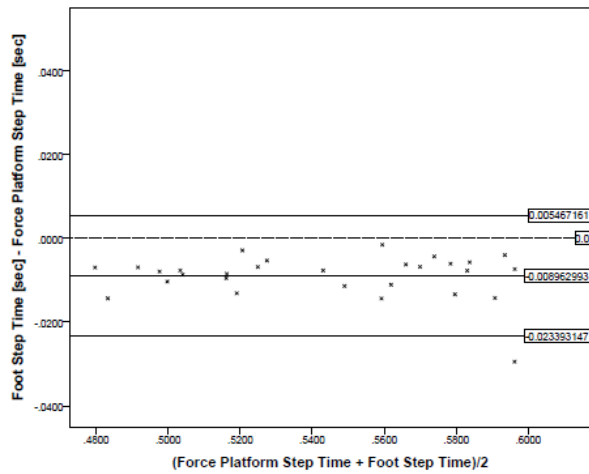
Figure 3. Bland-Altman plot comparing step time from the force plate and the foot IMUs.
