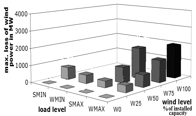
Fig. 3 – Maximum wind power contingency size following widespread voltage dip of 35% of nominal value
