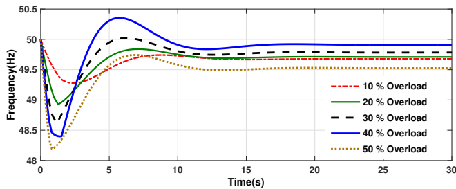
Figure 11. System frequency response using Increasing UFLS plan
