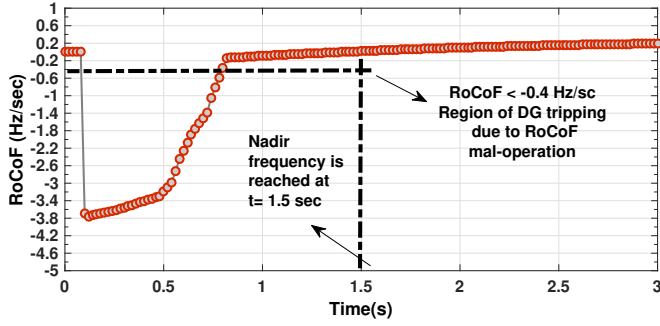
Figure 4. RoCoF variations using deterministic UFLS strategy
