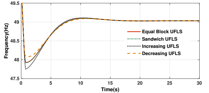
Figure 6. System frequency response using four UFLS strategies
