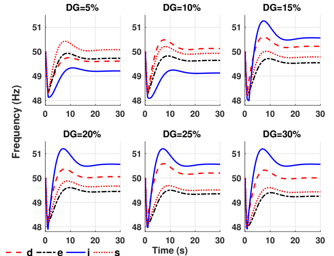
Figure 8. Comparison between Decrease (d), Increase (i), Sandwich (s) and equal (e) load shedding plans for 30% contingency
