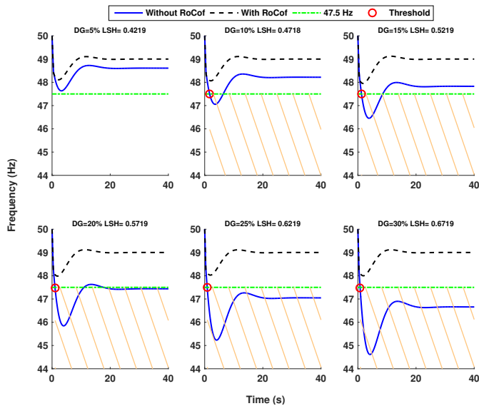
Figure 7. System frequency response under different values of DG penetration, With/without malfunction of RoCoF Relays for 50 % contingency
