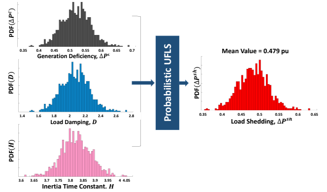
Figure 5. PDFs of inputs and output variables for IEEE-39 bus grid
