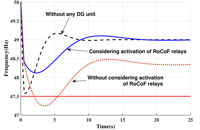
Figure 3. System frequency response using deterministic UFLS
