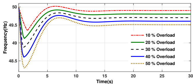
Figure 10. System frequency response using Equal Block UFLS plan
