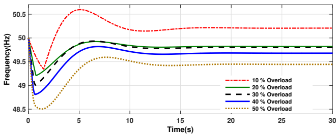
Figure 12. System frequency response using Decreasing UFLS
