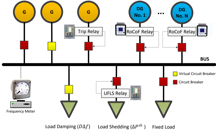
Figure 1. Sources of load and generation changes in system frequency response
