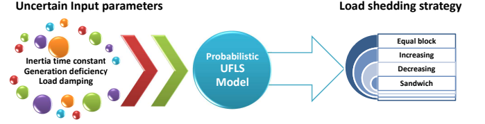
Figure 2. Inputs and outputs of the proposed probabilistic UFLS plan
