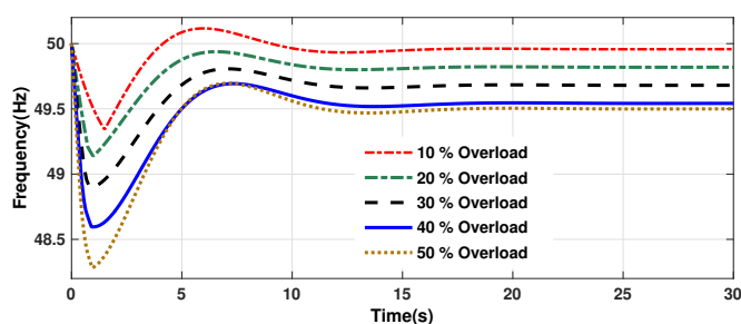
Figure 9. System frequency response using Sandwich UFLS plan
