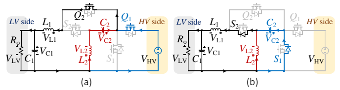
Fig. 3. Equivalent circuit of the proposed converter in step-down mode: (a) state 1 and (b) state 2.
