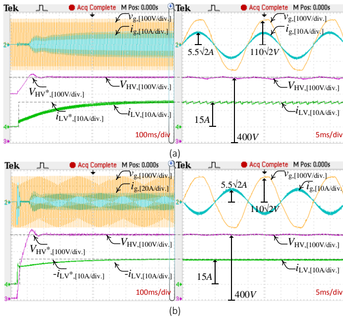
Fig. 16. Grid connected operation during: (a) V2G and (b) G2V.
