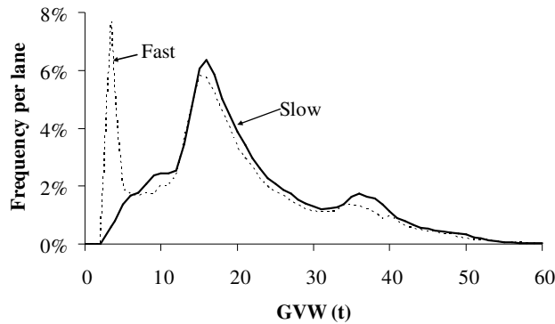
(a) Netherlands up to 60 t [132 kips].
