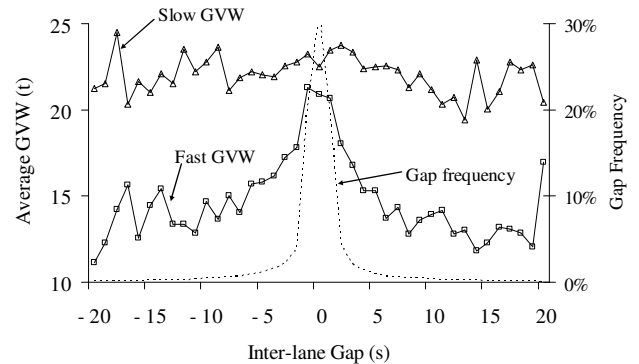
Figure 2. Inter-lane GVW correlation, the Netherlands.
