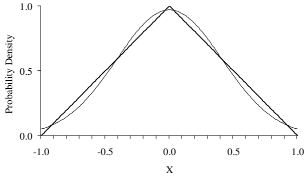
Figure 4. Normal and triangle kernel functions.
