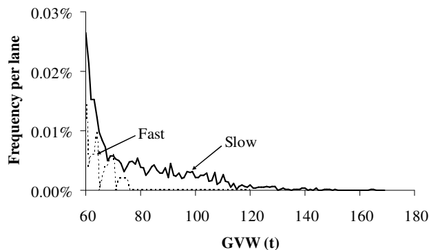
(b) Netherlands over 60 t.
