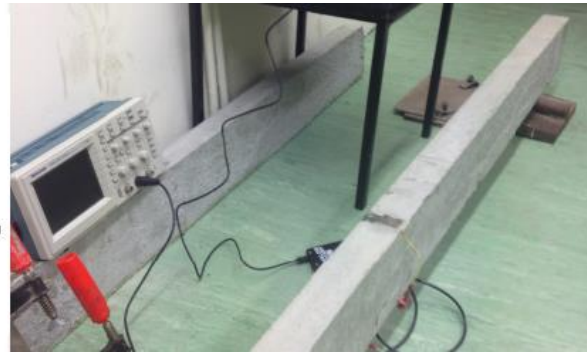
Figure 3. (a) Position of Energy Harvester and Damage Location (b) Experimental Setup
