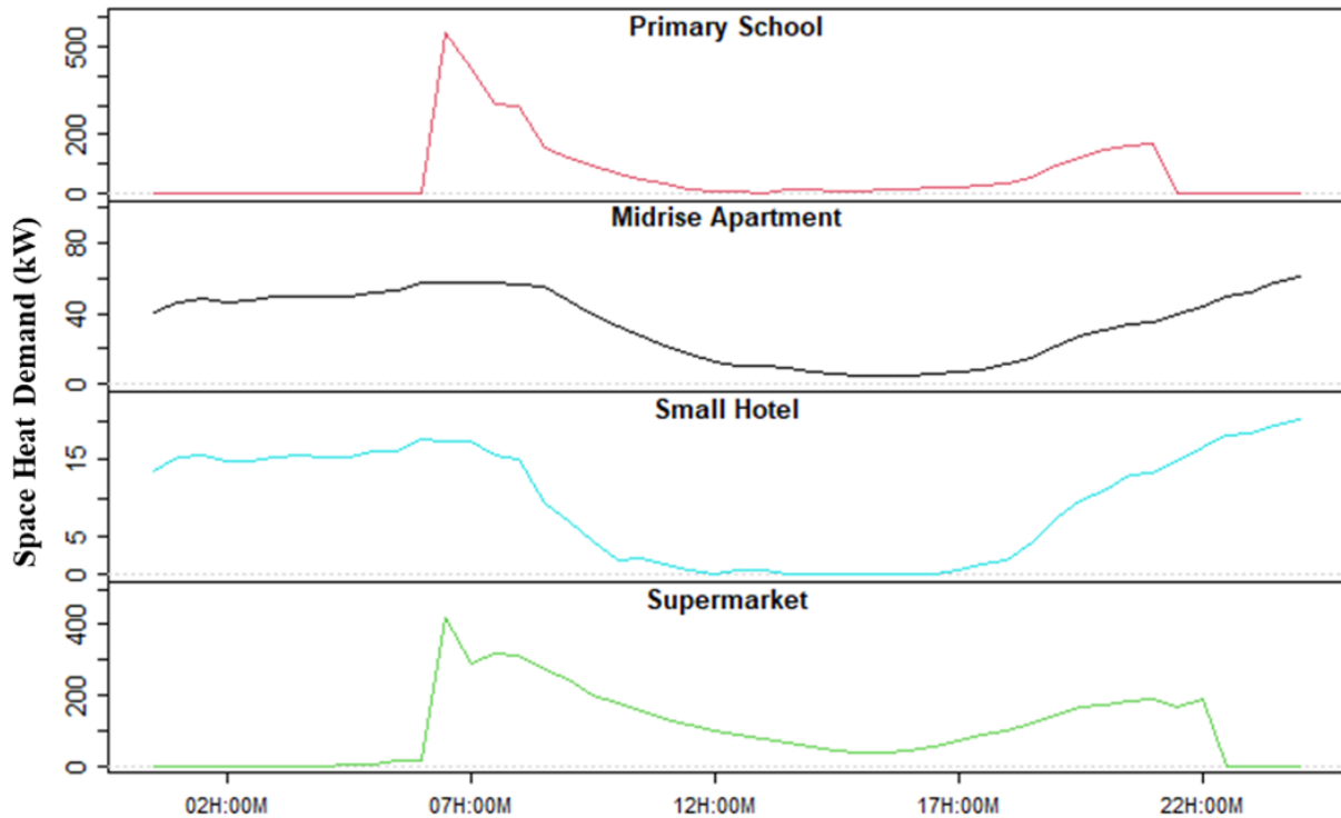
Figure 14: Daily heat demand profile for primary school, mid-rise apartment, small hotel and supermarket DOE reference buildings for possible interoperability characterisation.
