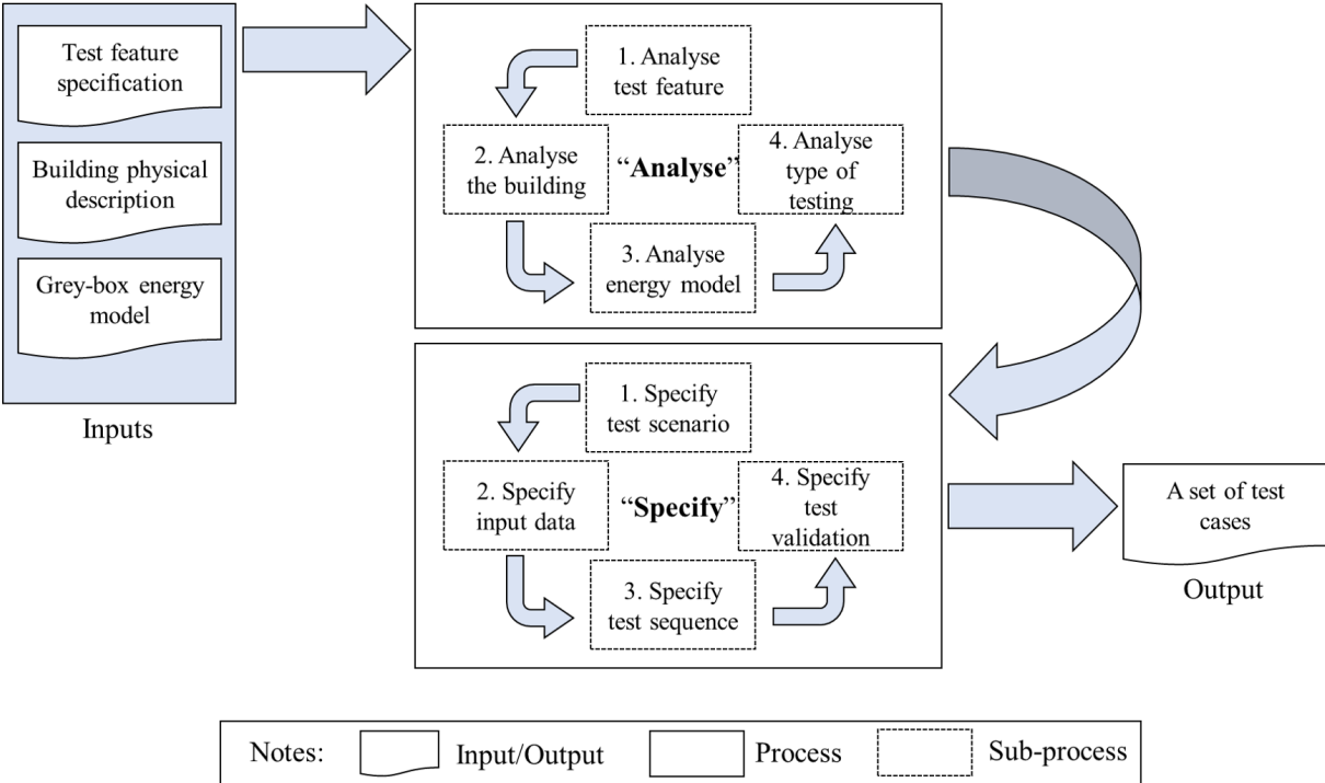
Figure 4: Model feature testing implementation process to identify the required experimentation for individual features.
