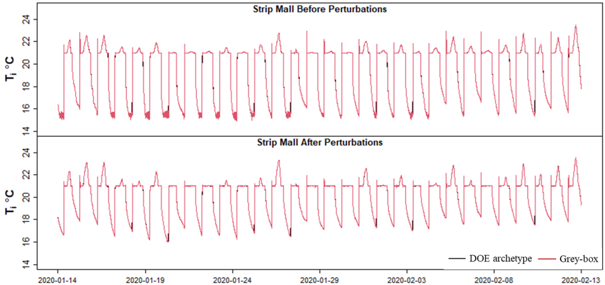
Figure 12: DOE archetype and grey-box internal temperature profiles for the strip mall DOE archetype at the whole building level before and after the introduction of design perturbations over a four week period.
