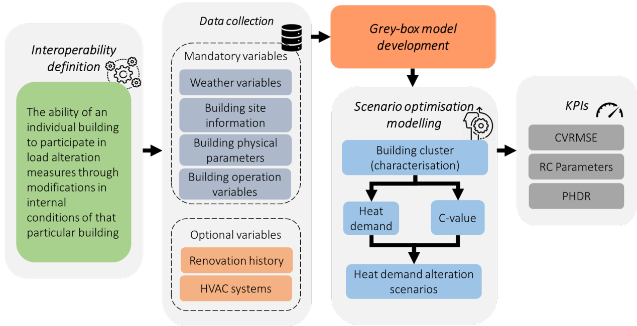
Figure 13: Interoperability assessment framework (sub-methodology) for reduced-order grey-box models.
