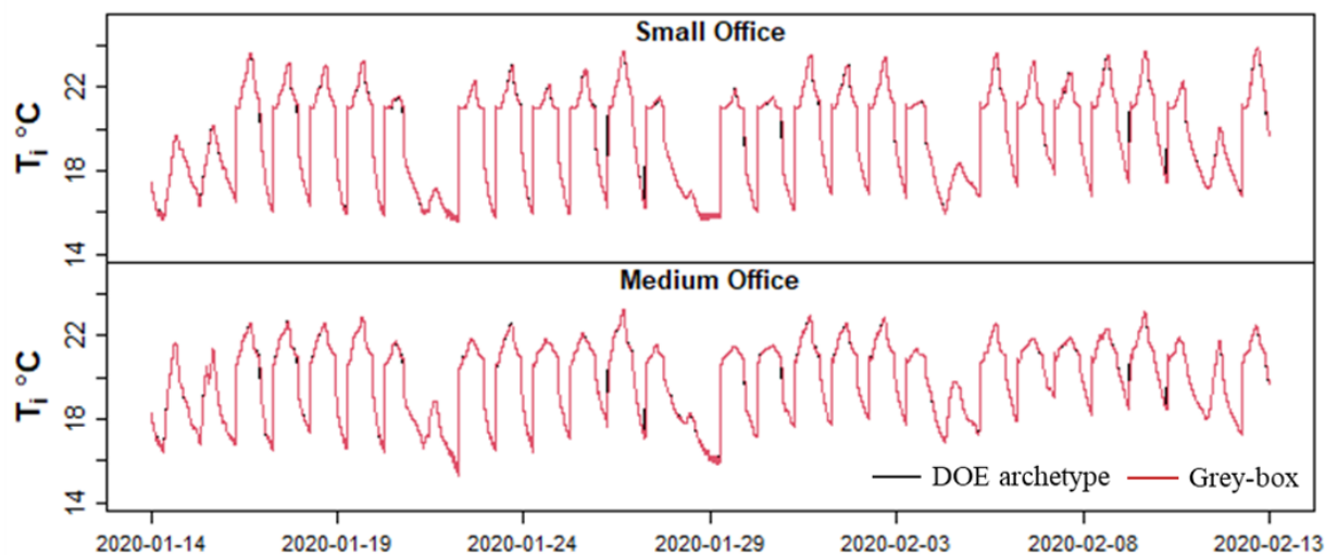
Figure 10: DOE archetype and grey-box internal temperature profiles for the small office and medium office DOE archetypes at the whole building level over a four week period.
