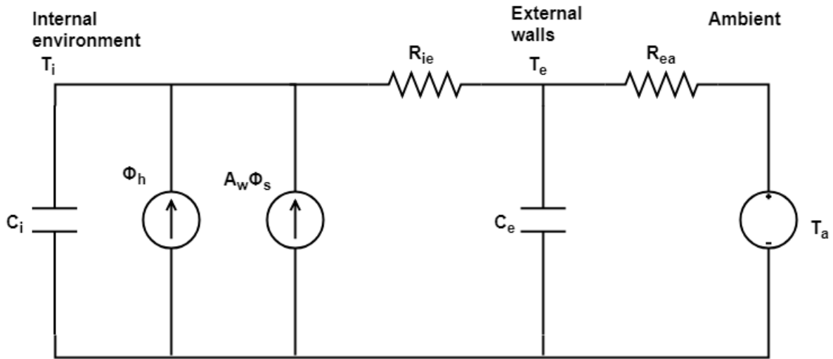
Figure 8: The implemented second order network for the small office DOE reference building. T_i , T_e and T_a represent the states of the internal, special zone, heater, exterior and ambient elements in the network. R_{ie} and R_{ea} represent the thermal resistances of the network. C_i and C_e represent the thermal capacities of the network. \phi_h and \phi_s are the heater and solar radiation flux elements. A_w represents the effective window area
