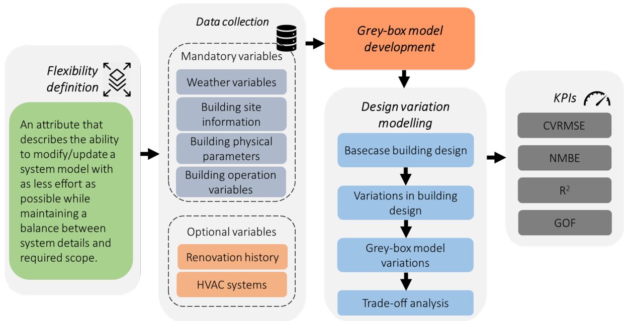
Figure 11: Flexibility assessment framework (sub-methodology) for reduced-order grey-box models.
