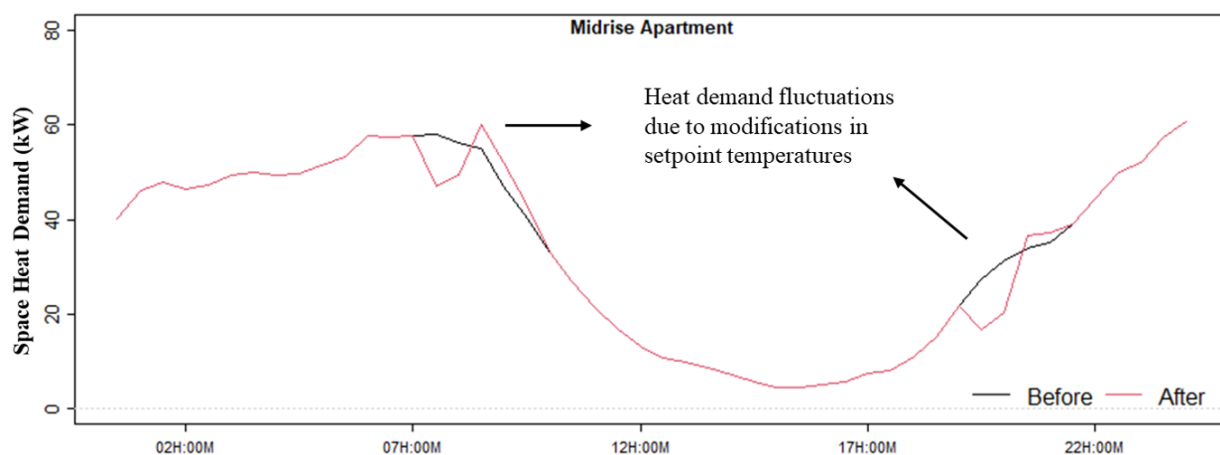
Figure 15: Daily heat demand profile for the midrise apartment DOE reference building before and after the introduction of demand alteration scenarios. The heat demand fluctuations represent time instants when the set-point temperature is varied.
