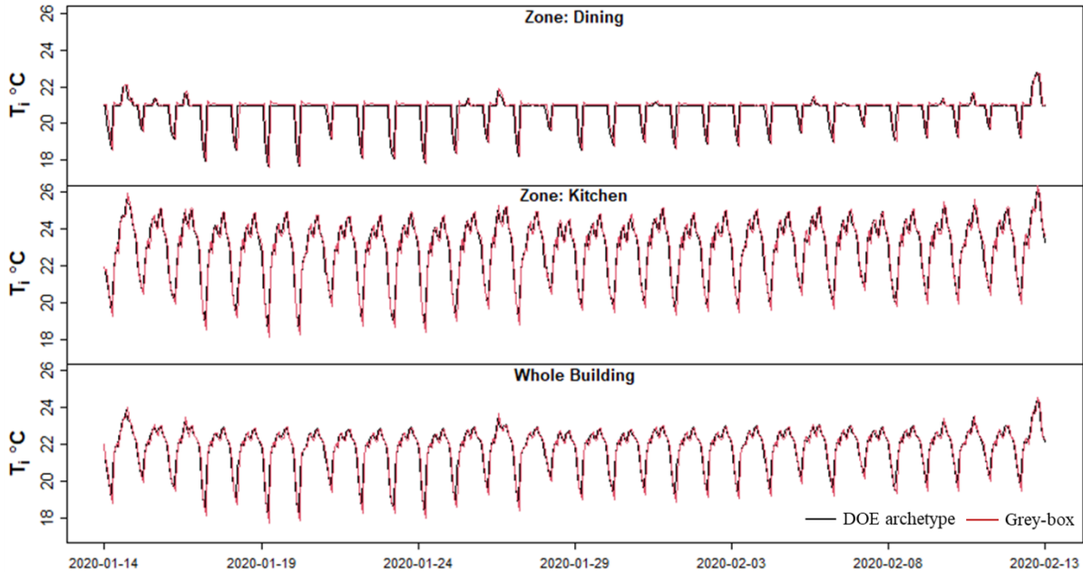
Figure Appendix B.1: DOE archetype and grey-box internal temperature profiles at the whole building level and respective zone level for the full service restaurant DOE archetype over a four week period.
