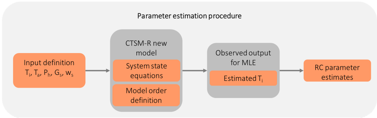
Figure 3: Parameter estimation procedure using CTSM-R to identify the thermal resistance and thermal capacitance values.
