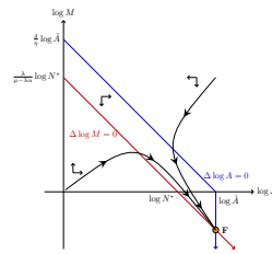
Figure 1: The four equilibria of the knowledge-misery system.
