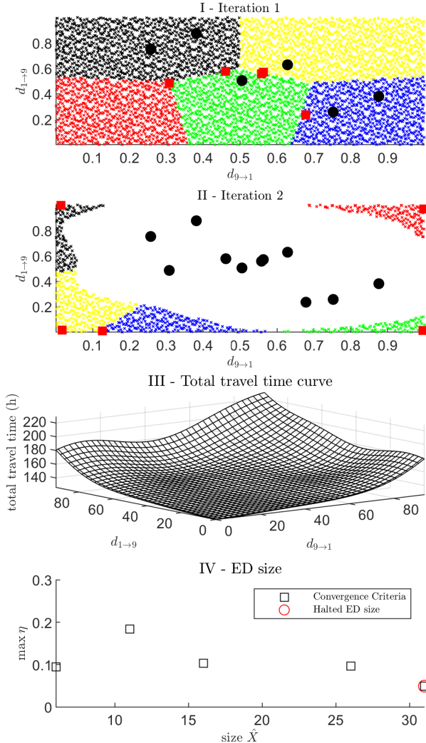
Figure 2: Example of metamodel fit to a two-dimensional example enclosing links 1 and 9 damage in the ED, respectively d_{1 \rightarrow 9} and d_{9 \rightarrow 1} , subscript node direction travel. I-II - Experimental design of iterations 1 and 2. III - Two-dimensional representation of the variations in travel time, depending on d_{1 \rightarrow 9} and d_{9 \rightarrow 1} . IV - ED size and relationship to the Sobol sequence in the present example metamodel definition.
