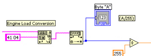
Figure 3: Data parsing and scaling of engine load.
