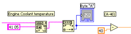
Figure 7: Data parsing and scaling function for engine coolant temperature.
