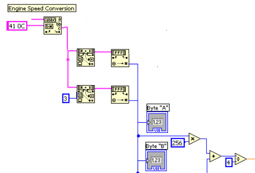
Figure 2: Data parsing and scaling function for engine speed.
