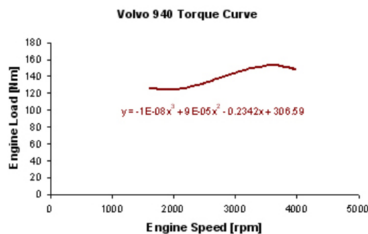
Figure 4: Torque curve for the Volvo 940. This digitised plot was used to determine the maximum load value for parsing.
