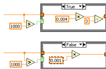
Figure 10: Implementation of the calculation scheme to determine the column identifier for both the range 0-999 rpm (above) and 1000-5500 rpm (below).
