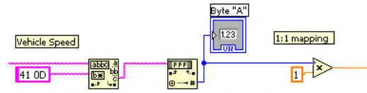
Figure 6: Data parsing and scaling function for vehicle speed. Notice the direct one-to-one mapping of the extracted byte value and the vehicle speed.
