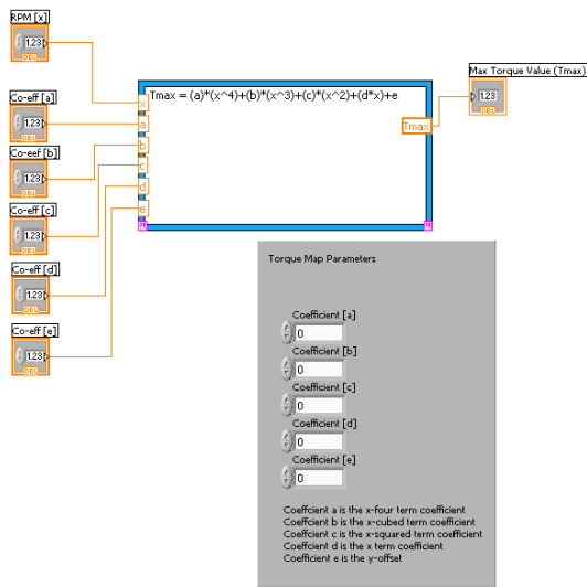
Figure 5: An implementation of the maximum torque curve method as employed in Version 2.0.1. The cumbersome nature makes it unwieldy as does the slow calculation using the MathScript Node.
