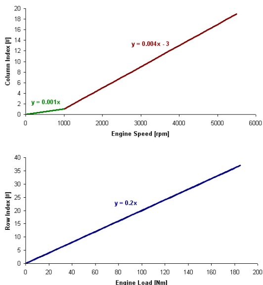
Figure 9: Graphical representation of the conversion equations used for (top) engine speed and (bottom) engine load for the bilinear interpolation VI.
