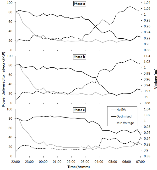
Fig. 9. Power delivered to network on each phase for the case with no EVs charging and the optimised charging case employing the standard objective function (Winter). The lowest CPOC voltage for each phase at each time step for the optimised charging case is also shown.
