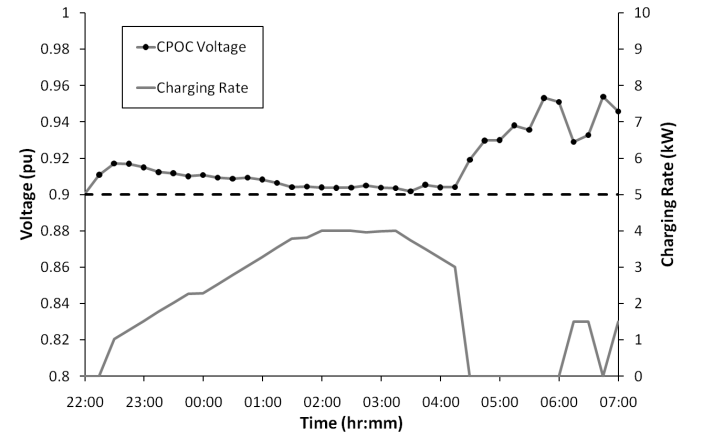
Fig. 11. Voltage profile for a CPOC at node 6 and charge profile for EV charging at the same CPOC with optimised charging employing the weighted objective function. (Winter scenario)
