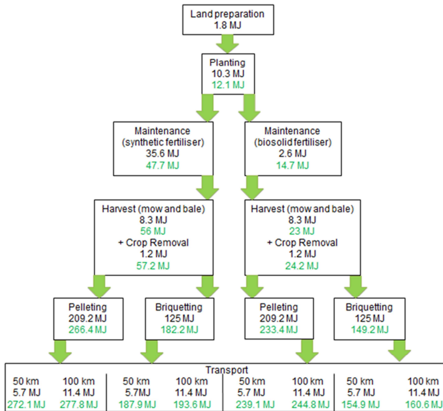
Figure 3 - Energy requirements of life cycle stages (MJ per GJ of energy produced)
