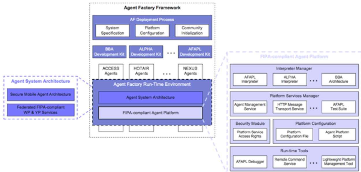
Figure 3: A Schematic of the Agent Factory framework
