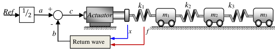
Fig. 1: WBC of rectilinear system without external disturbances: x = c = a + b = \frac{1}{2}r + b
