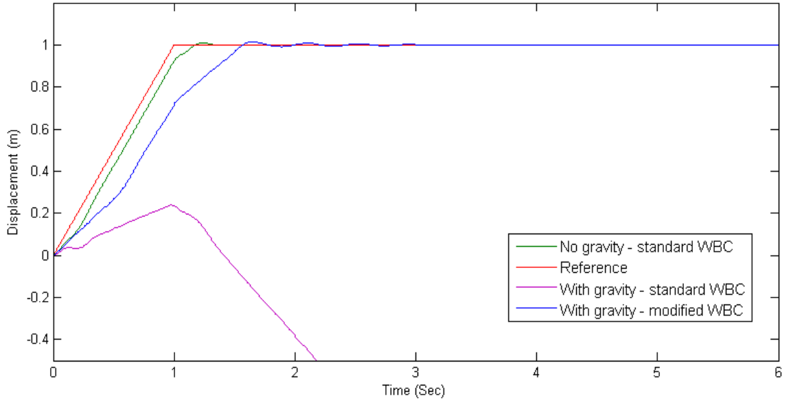
Fig.6: WBC response to slewing reference motion, with and without gravity, using standard WBC, Eq.(2), and modified, Eq.(4).
