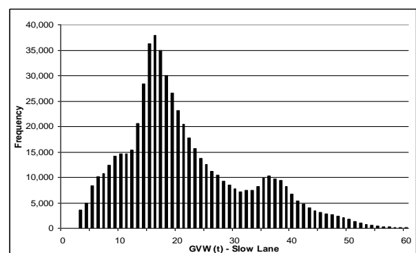
Figure 1. GVW Distribution 0t to 60t – Slow Lane
