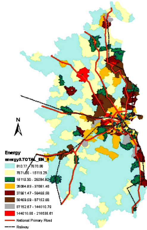
Figure 2 – Total energy demand at DED level, 2006
