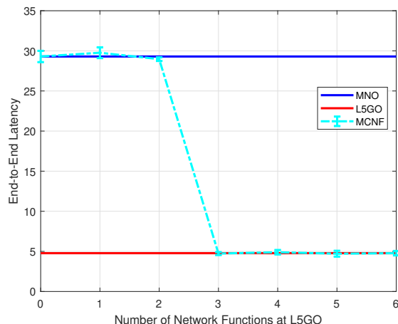
Fig. 21: Average AR packet latency under MCNF algorithm
