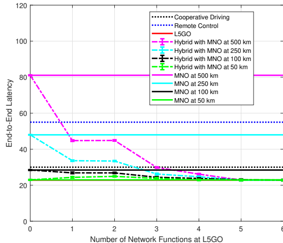
Fig. 30: Average packet latency of mobile robots use case under PP algorithm
