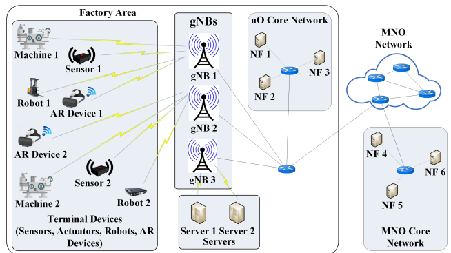
Fig. 19: Hybrid deployment model to serve factory use cases
