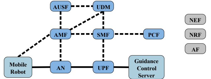
Fig. 13: Architectural components of L5GO to serve the mobile robots use case
