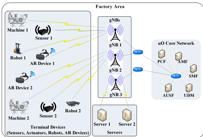
Fig. 16: Deployment model for pure local operator serving the factory use cases
