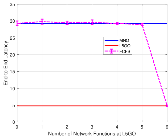
Fig. 20: Average AR packet latency under FCFS algorithm
