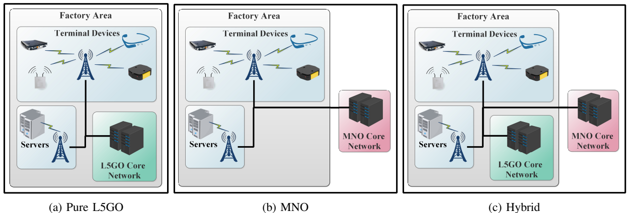
Fig. 15: Architectural Options
