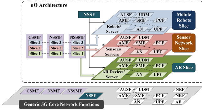
Fig. 14: Proposed architecture of L5GO with three network slices
