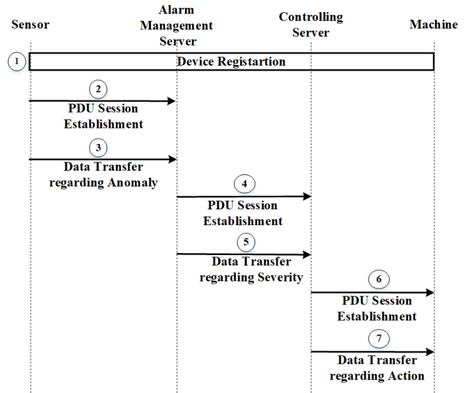
Fig. 10: Message sequence chart for emergency action based on sensor detection
