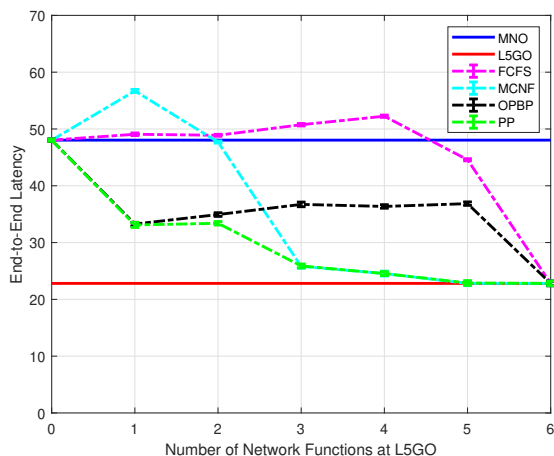
Fig. 26: Average packet latency of mobile robots use case
