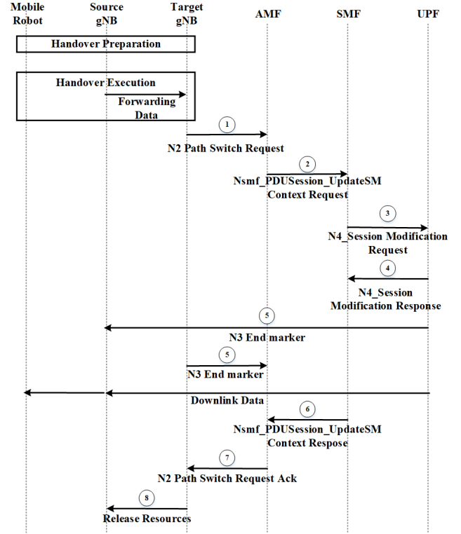
Fig. 12: Message sequence chart for handover procedure of robots
