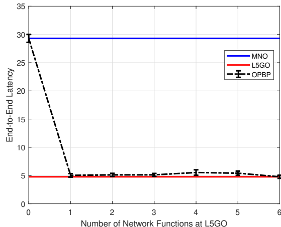
Fig. 22: Average AR packet latency under OPBP algorithm
