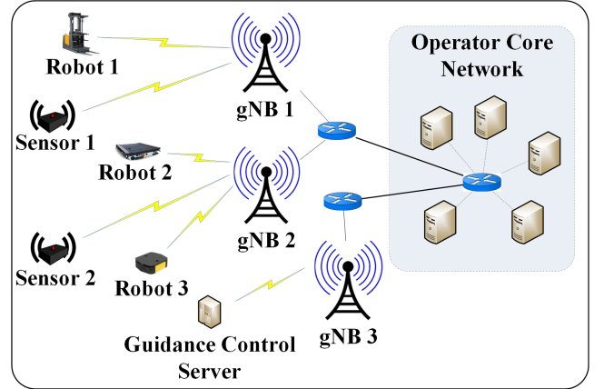
Fig. 6: Mobile robots controlled by a guidance control server
