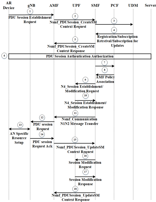
Fig. 8: Message sequence chart for session establishment between AR device and server
