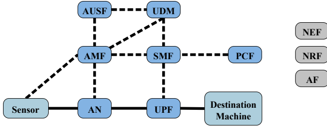
Fig. 11: Architectural components of L5GO to serve the massive wireless sensor networks use case
