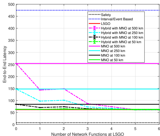
Fig. 29: Average packet latency of massive wireless sensor networks use case under PP algorithm
