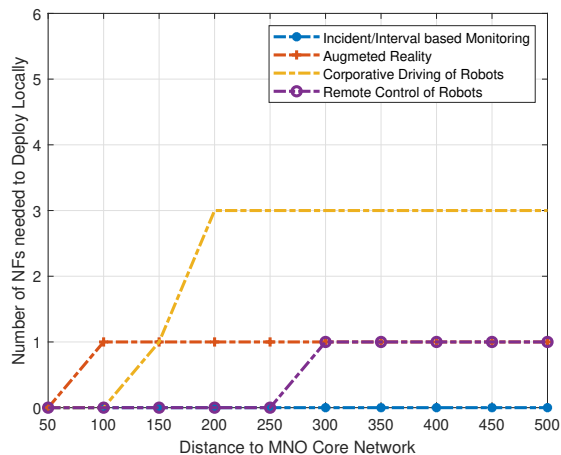
Fig. 31: Number of NFs needed with respect to d
