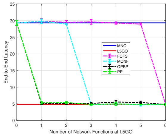
Fig. 24: Average packet latency of AR use case
