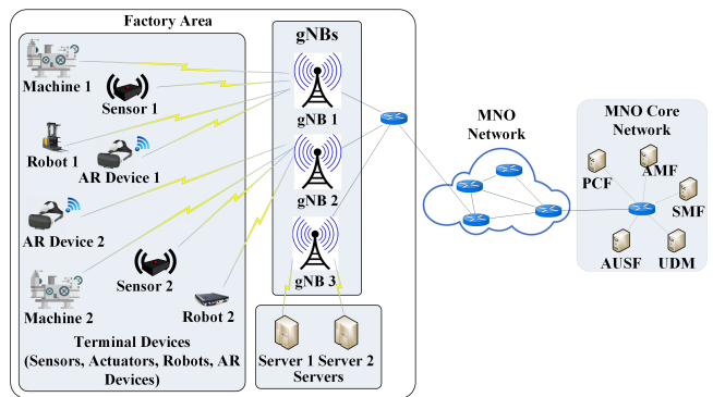
Fig. 18: Deployment model for MNO serving the factory use cases
