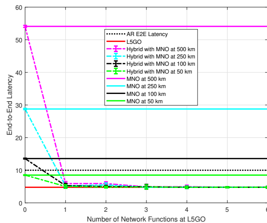
Fig. 28: Average packet latency of AR use case under PP algorithm
