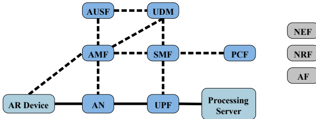
Fig. 9: Architectural components of L5GO to serve the AR use case
