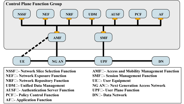
Fig. 1: Service based representation of 5G architecture [12]
