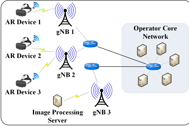
Fig. 4: An AR network with terminal devices and the AR server
