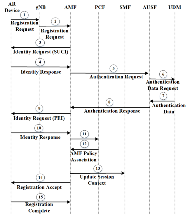
Fig. 7: Message sequence chart for AR device registration procedure
