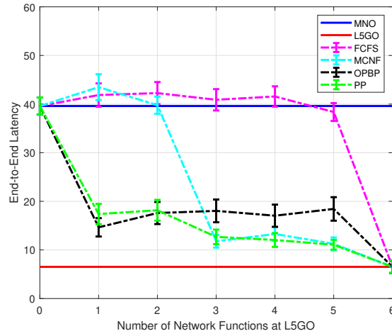
Fig. 27: Average packet latency combining all three use cases
