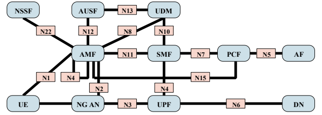
Fig. 2: Reference point representation of 5G architecture [12]
