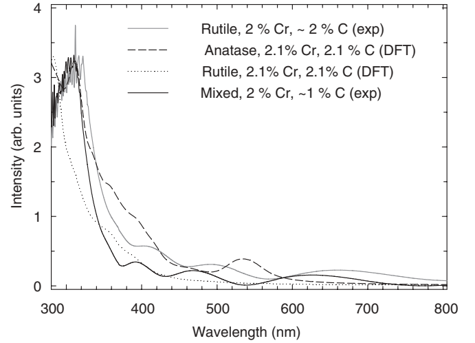
FIG. 13. Absorption spectra from experiment and DFT for Cr/C-codoped titania.
