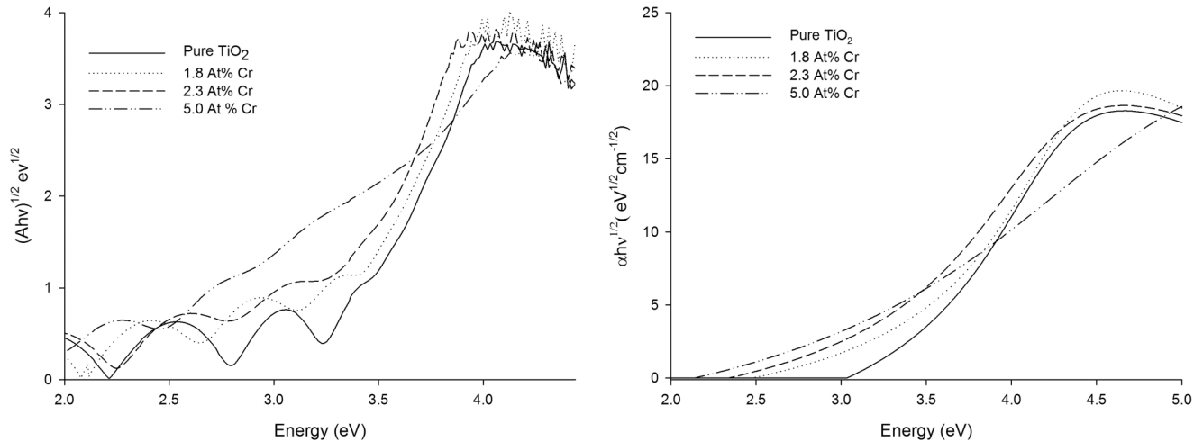
FIG. 6. Tauc plots of undoped and doped \text{TiO}_2 with different Cr-dopant concentration measured using UV-vis (left) and ellipsometry (right).
