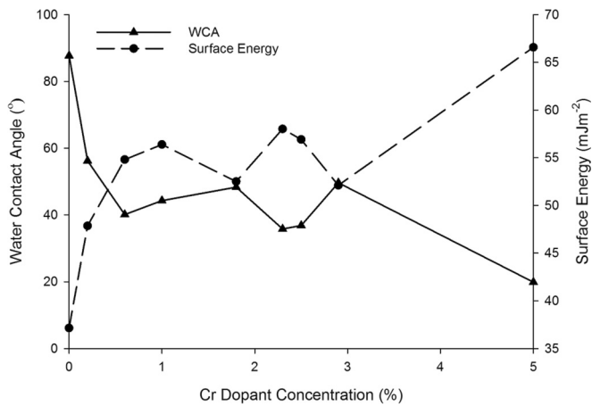
FIG. 2. Change in water contact angle (WCA) and surface energy values for various concentrations of Cr-doped \text{TiO}_2 .
