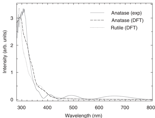
FIG. 7. Absorption spectra from experiment and DFT for pure titania.
