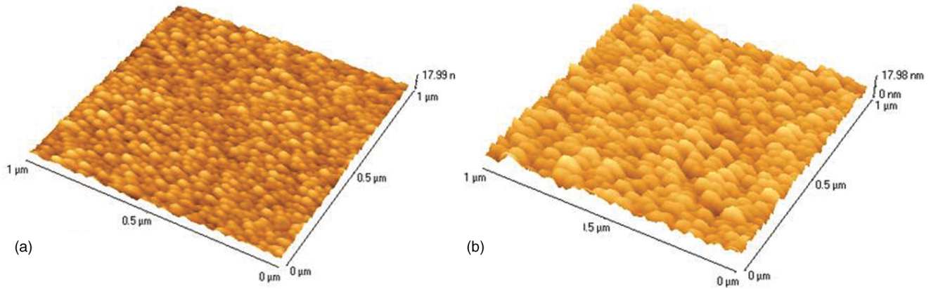
FIG. 4. (Color online) AFM topographical morphology of (a) undoped and (b) 5 at% Cr-doped sputtered-deposited TiO 2 coating.
