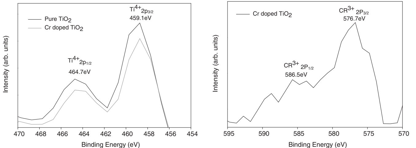
FIG. 1. XPS profiles of the binding energies for \text{TiO}_2 (left) and \text{Cr}^{3+} (right).
