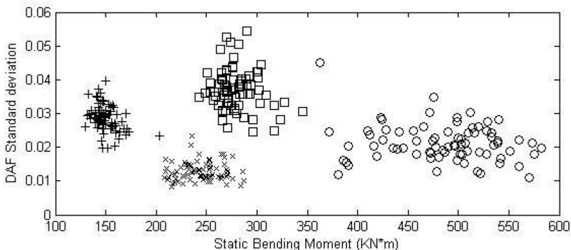
Figure 6. Standard deviation DAF value for each vehicle. 5-axle & 15m (+), crane & 15m (x), 5-axle & 25m (□), crane & 25m (○).
