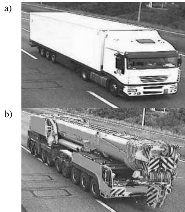
Figure 1. Photo examples of recorded WIM trucks, a) 5-axle truck, b) crane.
