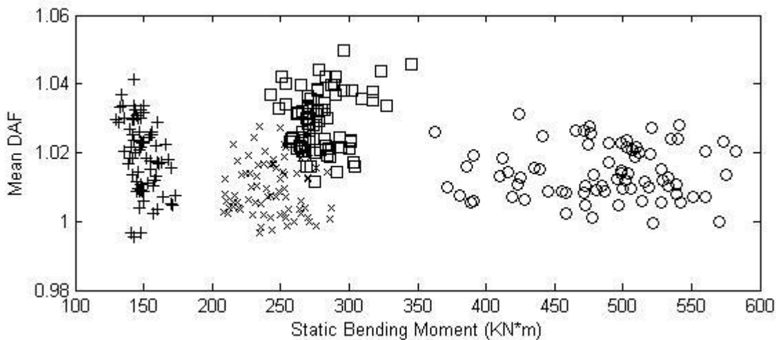
Figure 5. Mean DAF value for each vehicle. 5-axle & 15m (+), crane & 15m (x), 5-axle & 25m (□), crane & 25m (○).
