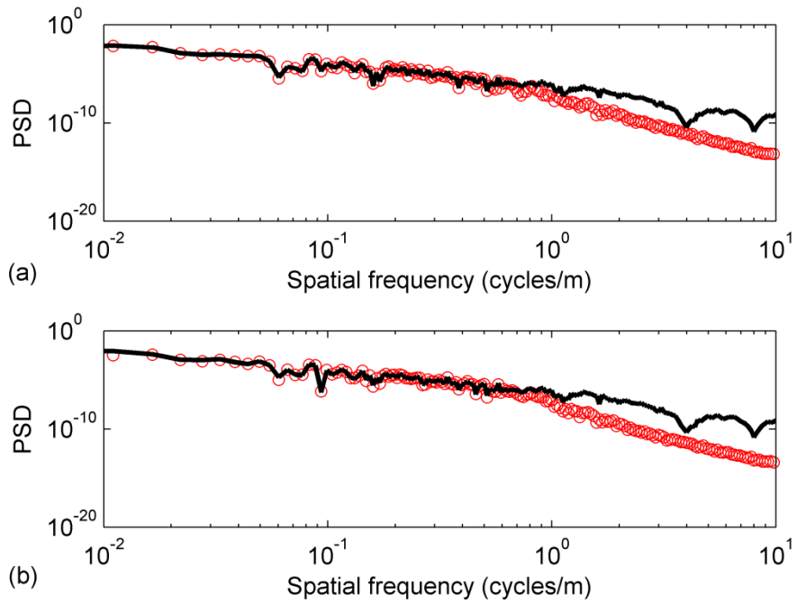
Fig. 9 PSD of average road profile heights under (a) wheel 1 and (b) wheel 2 for SNR = 10.
