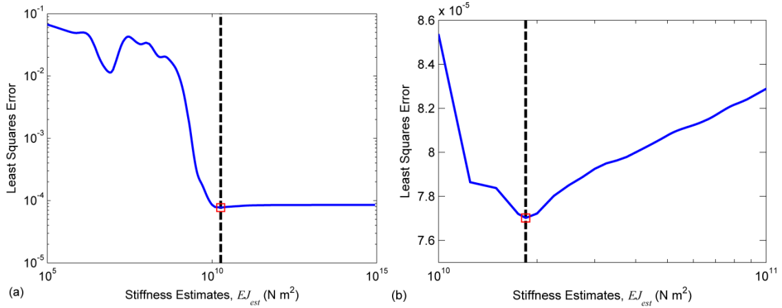
Fig. 11 (a) Least squares error, r_{error} (—) versus global stiffness estimates ( EJ_{est} ) for 15 m bridge span with SNR = 20, (b) same graph, zoomed in at minimum (□). Target stiffness value is 1.846 \times 10^{10} \text{ N m}^2 (---).
