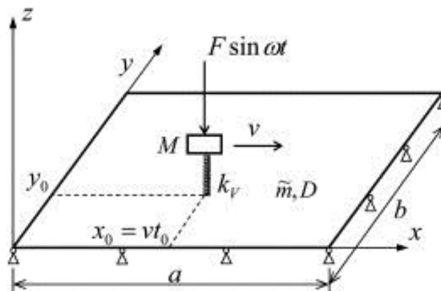
Figure 5: A passing tapping vehicle on a plate [43].
