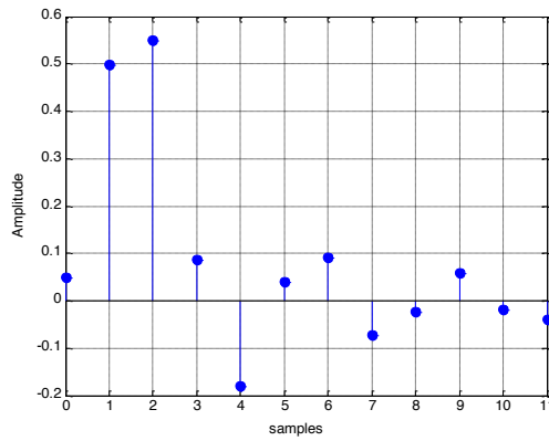
Figure 5. Case study filter impulse response.
