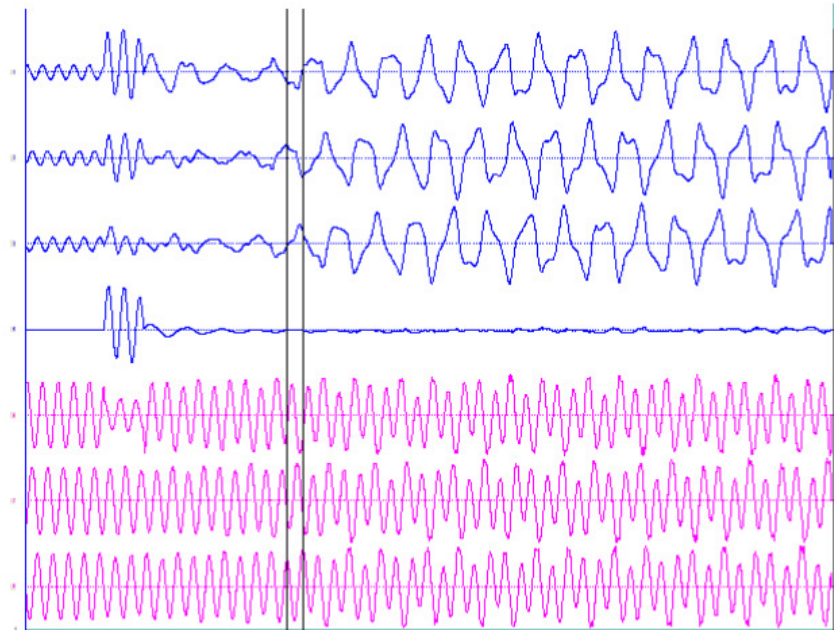
Fig. 11: Measured quantities (phase currents (top - blue) and voltages (bottom - magenta)) at receiving end of transmission line in ERCOT system. Source: Electranix
