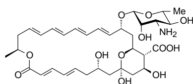
33 4, 5 De-epoxypimaricin
