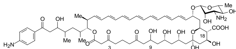
5 Candicidin
