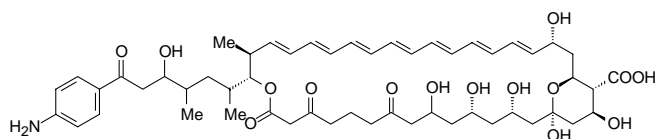
31 FR008 VII
