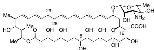
3 Amphotericin A
