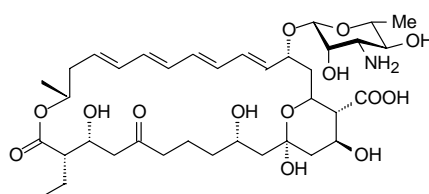
7 CE-108
