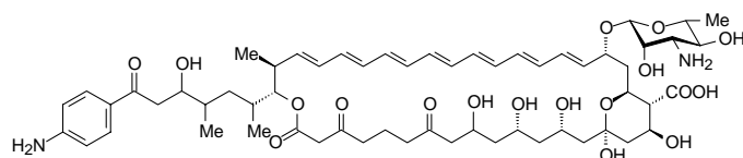
29 FR008-III
