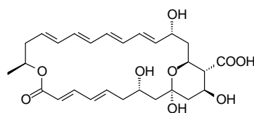
34 4, 5 De-epoxypimaricinolide
