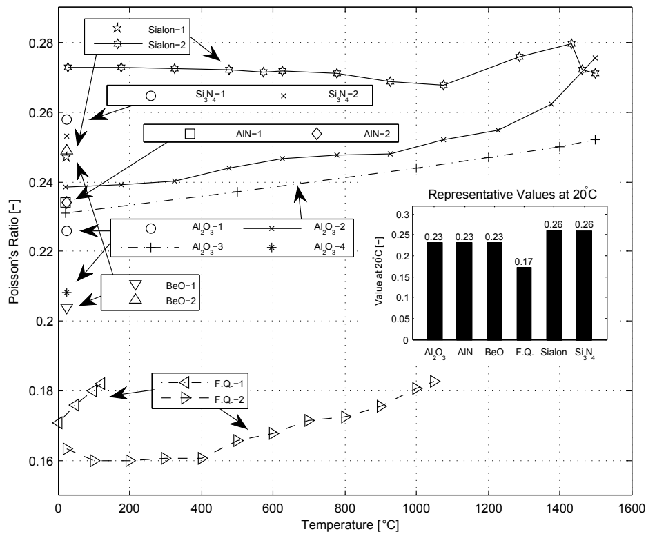
Fig. 5 Poisson's ratio values from the following references: \text{Al}_2\text{O}_3 -1 CoorsTek AD995 alumina [100]; \text{Al}_2\text{O}_3 -2, near-theoretical density alumina [132]; \text{Al}_2\text{O}_3 -3, review of alumina [17]; \text{Al}_2\text{O}_3 -4, hot pressed & HIPped alumina [135]; AlN-1, Cercom HP AlN [98]; AlN-2, Dow Chemical Corporation HP AlN [148]; BeO-1, fully dense BeO [58]; BeO-2, single crystal BeO [149]; F.Q.-1, Toshiba Ceramics T-1030 fused quartz [106]; F.Q.-2, fused silica [140]; Sialon-1, Kennametal TK4 sialon [100]; Sialon-2, near-theoretical density \beta -sialon [132]; \text{Si}_3\text{N}_4 -1, Ceradyne Ceralloy 147-31N silicon nitride [100]; \text{Si}_3\text{N}_4 -2, Kyocera SN235P silicon nitride [100].
