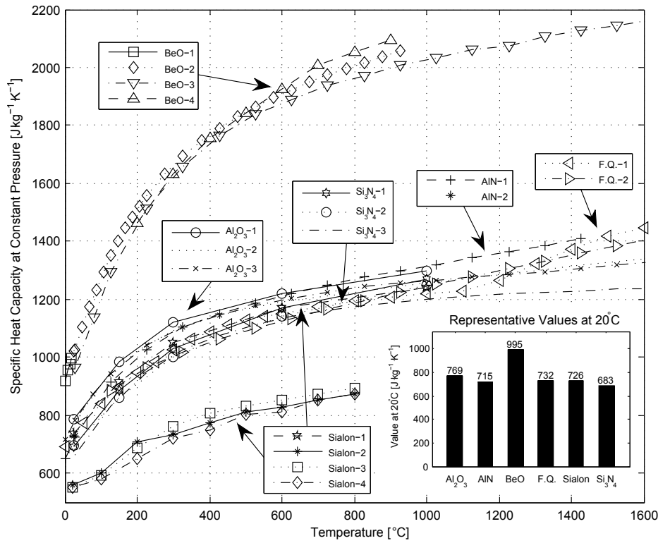
Fig. 9 Specific heat capacity values from the following references: Al 2 O 3 -1, CoorsTek AD995 alumina [100]; Al 2 O 3 -2, review of alumina [17]; Al 2 O 3 -3, review of alumina [170]; AlN-1, theoretical calculation for AlN [144]; AlN-2, theoretical calculation for AlN [171]; BeO-1, 99.6% pure BeO [172]; BeO-2, 99.96% pure BeO [173]; BeO-3, theoretical calculation for BeO [174]; BeO-4, beryllia [175]; F.Q.-1, review of vitreous silica [99]; F.Q.-2, review of vitreous silica [168]; Sialon-1, Kennametal TK4 sialon [100]; Sialon-2, 100 wt% \beta -sialon [78]; Sialon-3, 5 wt% \alpha -, 95 wt% \beta -sialon [78]; Sialon-4, 20 wt% \alpha -, 80 wt% \beta -sialon [78]; Si 3 N 4 -1, Ceradyne Ceralloy 147-31N silicon nitride [100]; Si 3 N 4 -2, Kyocera SN235P silicon nitride [100]; Si 3 N 4 -3, theoretical calculation for \beta -Si 3 N 4 [90].
