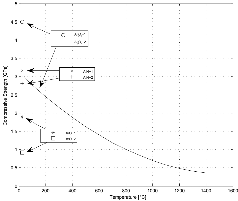
Fig. 8 Compressive strength values from the following references: Al 2 O 3 -1, hot pressed Al 2 O 3 [60]; Al 2 O 3 -2, review of alumina [17]; AlN-1, hot pressed AlN [60]; AlN-2, hot pressed AlN [167]; BeO-1, cold pressed & sintered BeO [60]; BeO-2, hot pressed BeO [60].
