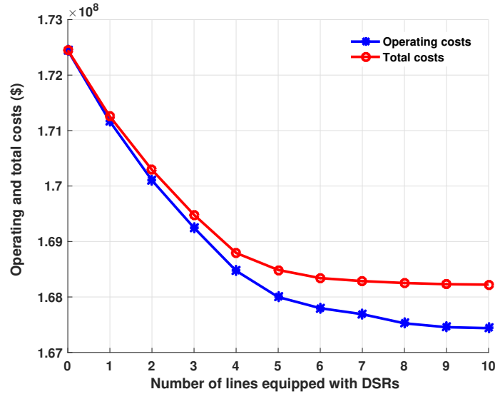
Fig. 7. Total cost and operating costs ($) vs number of lines equipped with DSR
