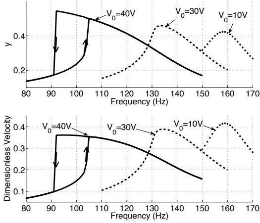
Figure 3: The resonant frequency shift, of the mass, due to electromechanical coupling. (a) describes the normalised displacement of the oscillating mass and (b) presents the change in the normalised velocity for the same electromechanical coupling.
