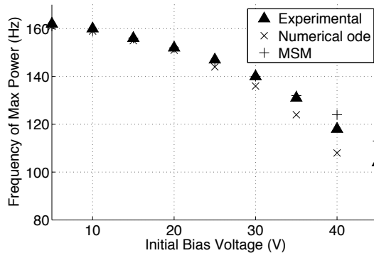
Figure 10: Comparison of the three models showing the frequency corresponding to the maximum power for a spectrum of initial bias voltages. The resistive load R_L was fixed equal to 8.9M\Omega . The appearance of hysteresis between V_0 = 35V and V_0 = 40V reduces the accuracy of the models due to the increased nonlinear nature of the system.
