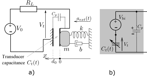
Figure 1: a) Block diagram of the continuous conditioning circuit. In this study the continuous circuit represents all circuit configurations which employ a capacitive transducer, resistive load and some internal or external voltage to provide the initial bias on the transducer. b) Equivalent schematic of a capacitive transducer biased by an electret layer.
