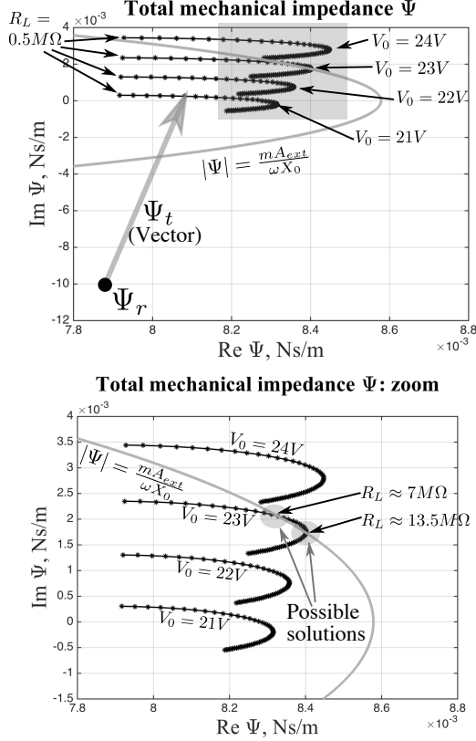
Figure 7: The loci of the total mechanical impedance of the system \Psi = \Psi_r + \Psi_t for different V_0 and R_L (black lines with stars). The grey line is the locus |\Psi| = \frac{mA_{\text{ext}}}{\omega X_0} . Each black line is plotted for the specified V_0 voltage, each star point in the line corresponds to a particular value of R_L . For each line, R_L varies on the grid (0.5,1...30) MΩ, the point with larger \text{Im}\Psi correspond to the smallest load resistance.
