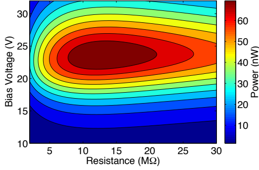
Figure 4: Global power maximum on a plane of R_L and V_0 , for fixed external vibrations ( A_{\text{ext}} = 0.25g and f_{\text{ext}} = 150Hz ). For the given external driving, the optimum is located at R_L = 13M\Omega and V_0 = 23.5V . It changes for different external excitations, limited only by the mechanical stoppers and pull-in between the capacitor plates.
