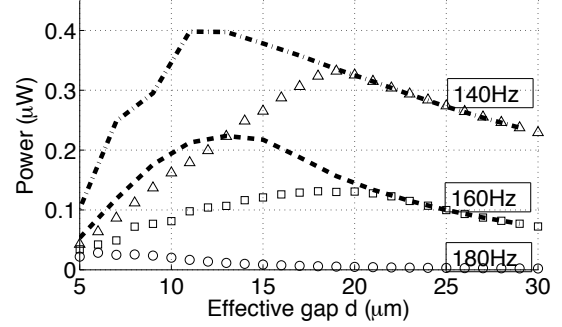
Figure 5: Optimum Power for the parameter space d , V_0 and R , for fixed external vibrations ( A_{\text{ext}} = 0.25gm/s^2 ). Lines denote unrestricted motion (140 and 160 Hz), where 160Hz is close to the natural resonance frequency of the unbiased mechanical resonator. The shapes detail the optimisation for the case when the mobile electrode motion is restricted to 0.75d amplitude (140, 160 and 180 Hz).
