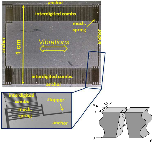
Figure 8: Picture of the fabricated device and a diagram explaining the profile of the transducer gap.
