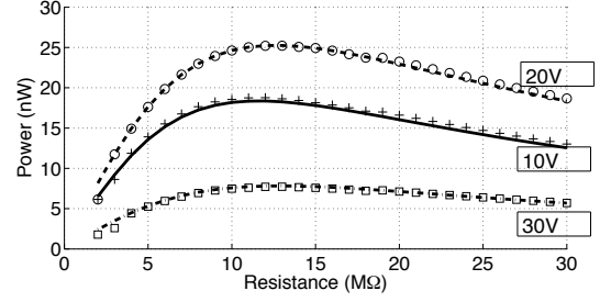
Figure 2: Harvested power versus load resistance for various bias voltages. Lines denote solutions of the MSM and characters present solutions of the system of ordinary differential equations (1)-(3). There is an optimum resistance for the continuous circuit, roughly 11MΩ in the presented case.
