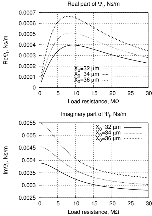
Figure 6: Result of electrical simulations of the conditioning circuit: real and imaginary parts of the transducer impedance for different load resistances ( R_L ) and amplitudes of displacement ( X_0 ), V_0 = 10V , with symmetrical gap closing transducer, with parameters given in Table 3.
