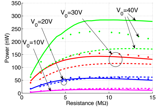
Figure 9: Validation of the proposed models with experimental data (dots). The numerical model is shown with full lines, and the MSM model is presented by dotted lines.
