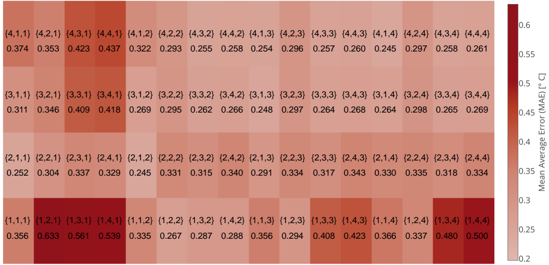
Figure 17: Mean Absolute Error ( MAE ) Heat Map, R_{ext1} as variable parameter (Simultaneous Calibration)
