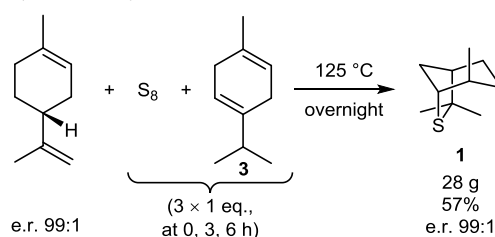
Scheme 2 Syntheses of isothiocieneole 1 .
