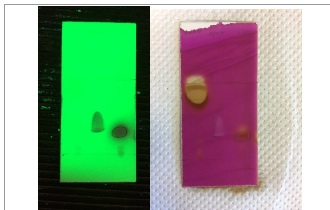
Figure 4 TLC monitoring of epoxidation reaction (pentane:ethyl acetate, 98:2); isothiocineole 1 R_t = 0.87 (left lane), epoxide 5 R_t = 0.50 (middle lane), benzaldehyde R_t = 0.32 (right lane), sulfonium salt 3 R_t = 0.00 . Visualized by UV light (254 nm; left plate) and KMnO 4 /NaOH (right plate).
