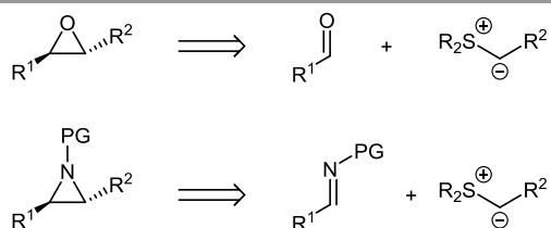
Scheme 1 The sulfur ylide disconnection for epoxides and aziridines.
