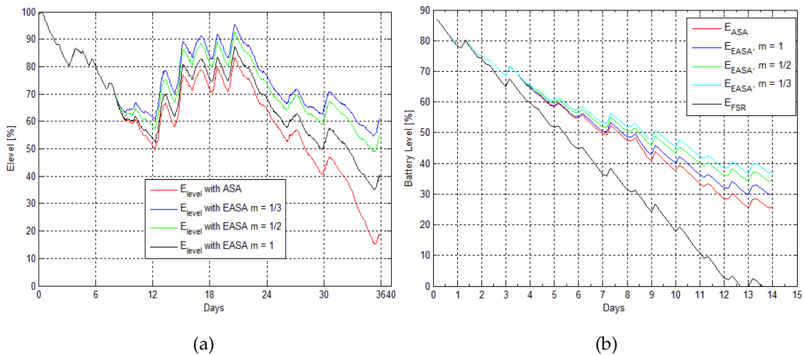
Figure 9. (a) Deployment (I) - Energy in the system (ASA vs. EASA) as a function of time; (b) Deployment (II) - Energy in the system (ASA vs. EASA) and fixed sampling rate energy level ( E_{FSR} ) as a function of time.
