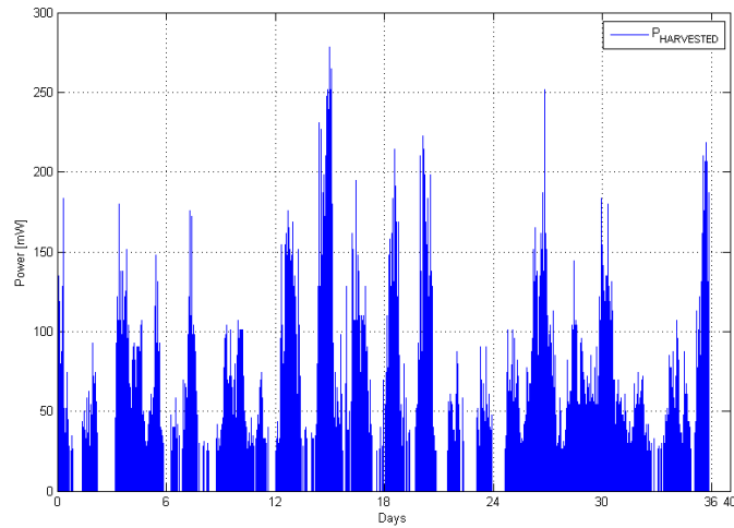
Figure 5. Harvested power from the wind during the 35 days of experiment -deployment (I).
