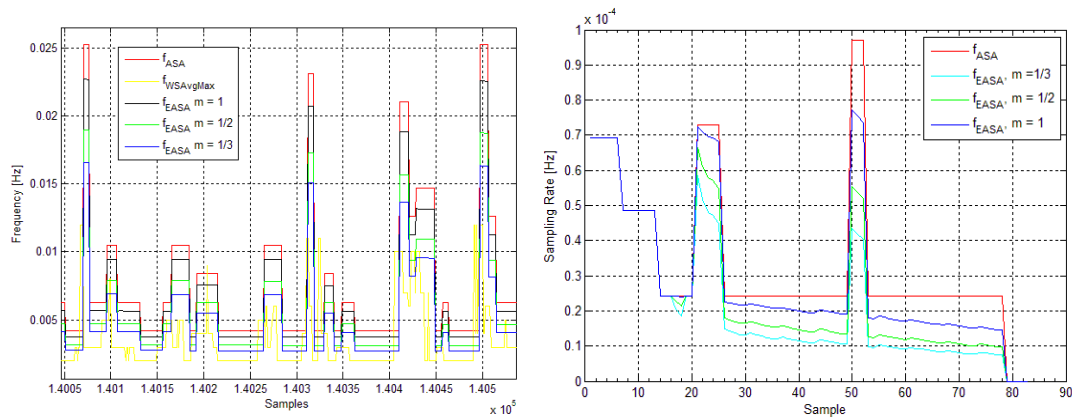
Figure 8. (a) Deployment (I) - Sampling rates and maximum frequency of the average wind speed signal vs. samples; (b) Deployment (II) - Sampling rates and maximum frequency of the average wind speed signal vs. samples.
