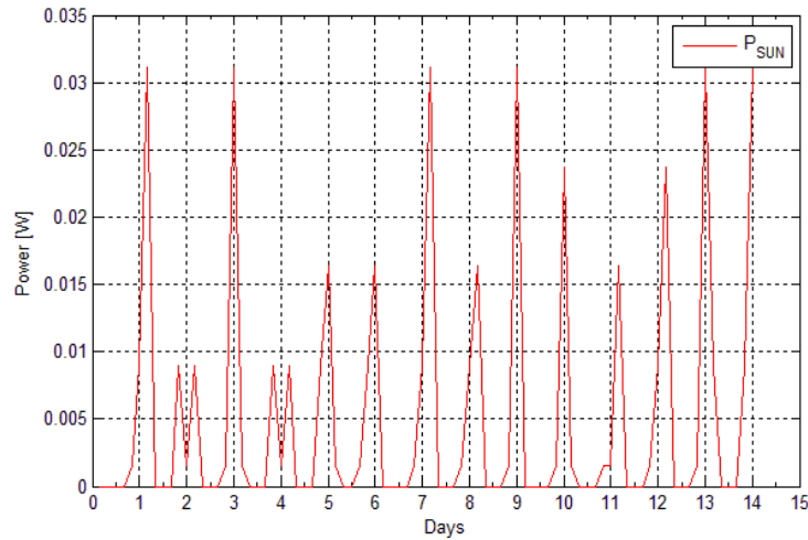
Figure 7. Harvested power from Sun -deployment (II).
