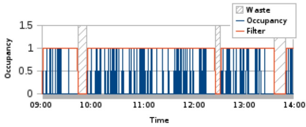
Figure 7. Private office presence detection with filter
