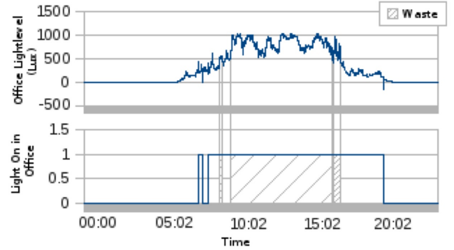
Figure 5. Open plan office ambient lighting levels compared to time lighting is activated over a 24hr. period
