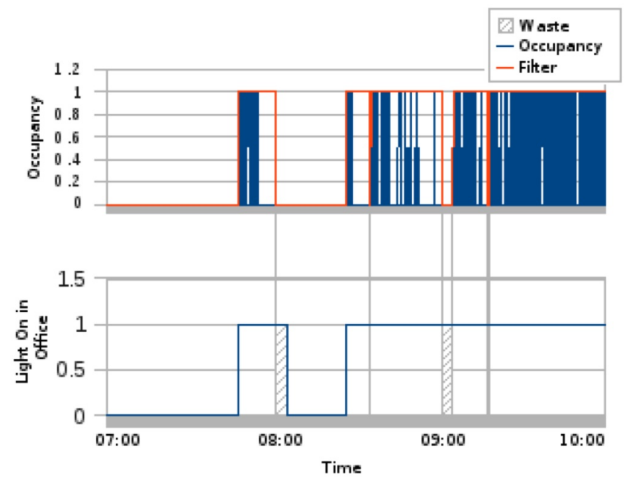
Figure 6. Open plan office presence detection with filter
