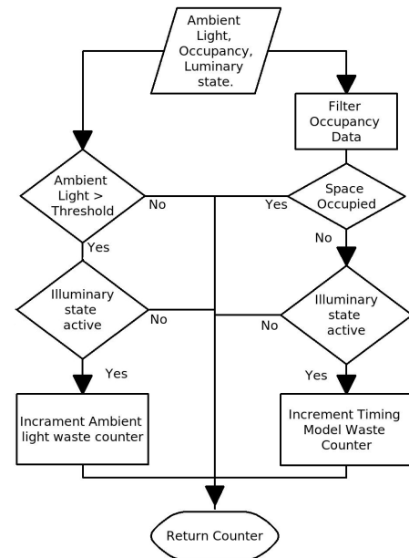
Figure 1. Process flow for modelling data
