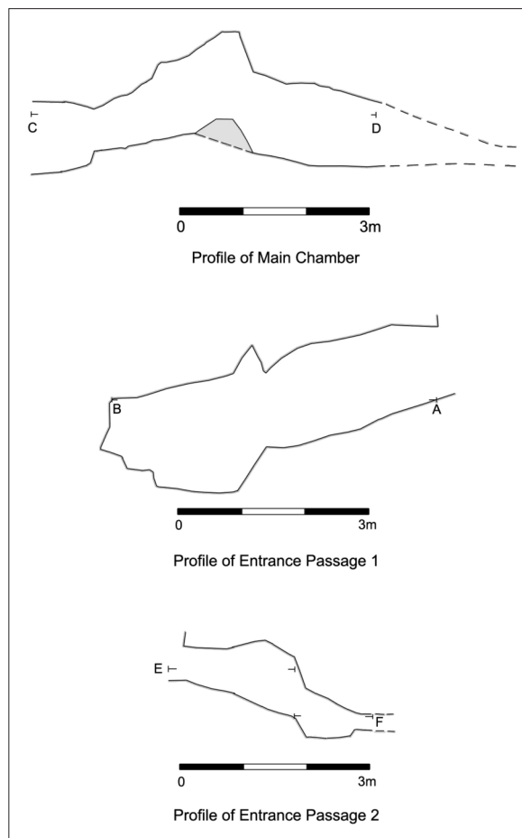
Fig. 5—Longitudinal profiles of the Main Chamber, Entrance Passage 1 and Entrance Passage 2 following the 1996 excavation (Sam Moore and Thorsten Kahlert).
