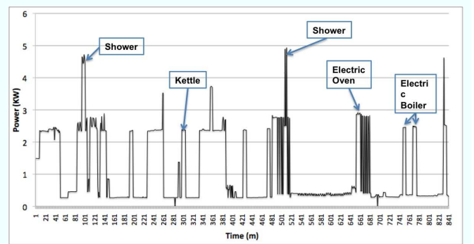
Fig. 1. Typical energy consumption in domestic premises
