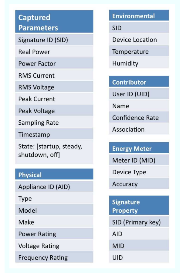
Fig. 5. Integration of unique signature state information
