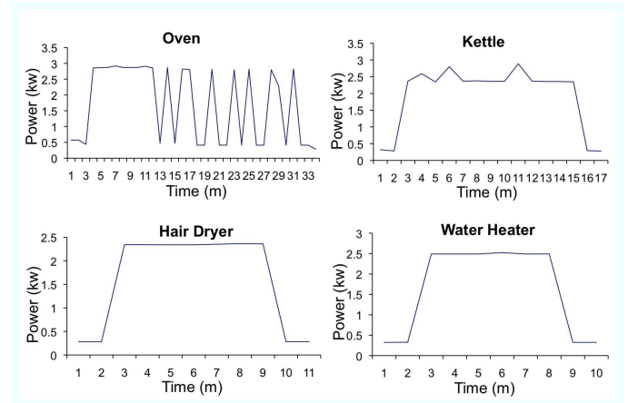
Fig. 4. Active Power Signatures for 4 appliances
