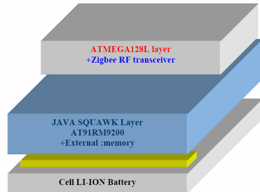
Figure 4. Agent Ready System Block diagram
