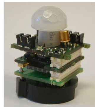
Figure 5. 25mm BEM Standard Sensor Layer
