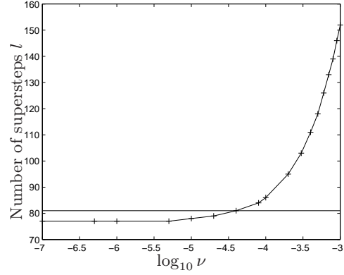
(b) Number of supersteps l versus \log_{10} \nu
