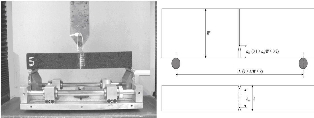
Figure 4 (a) View of 3PB loading fixture. Specimen length and height were 260mm and 40mm, respectively. (b) Schematic representation of a SENB test specimen with side grooves. (Top) Front view. (Bottom) Top View. Dimensions used in this work L = 240\text{mm} , W = 40\text{mm} , b = 20\text{mm} , b_n = 16\text{mm} , a_0 = 8\text{mm} .
