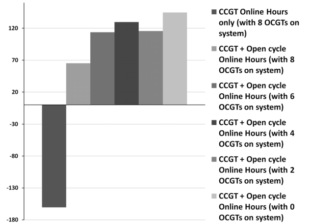
Fig. 3. Change in average number of online hours for CCGT 3 and 4 resulting from facilitation of multi-mode CCGT operation, shown for various generation portfolios
