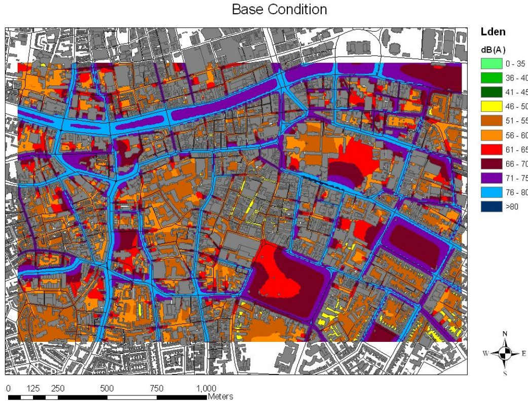
Figure 6: Noise Map for Dublin City Centre – base condition.
