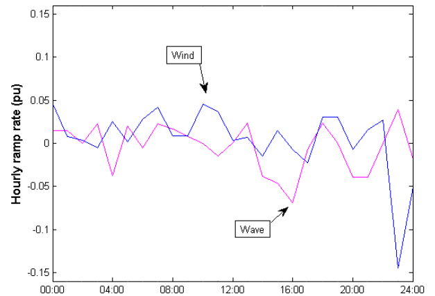
Fig. 13 Hourly variation across one day in January for system-wide wind ramp rates and for an aggregate of wave data from buoys M3 and M6
