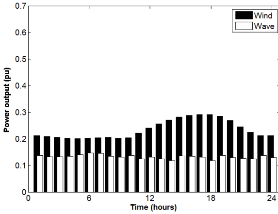
Fig. 9 Average hourly normalised system-wide wind generation and a non-downrated device wave farm at buoy M3 during quarter 2
