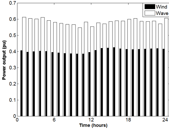
Fig. 8 Average hourly normalised system-wide wind generation and a non-downrated device wave farm at buoy M3 during quarter 1
