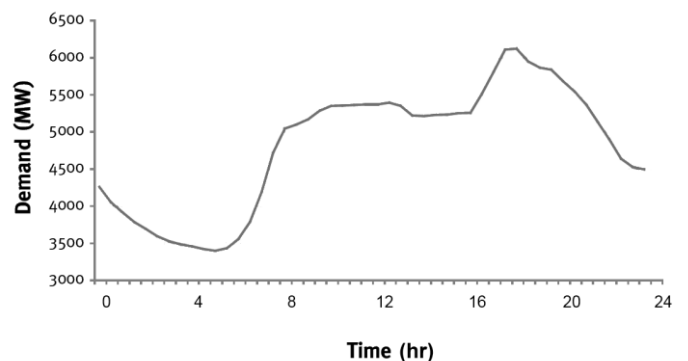
Fig. 1 A typical daily demand curve in Ireland in Winter
