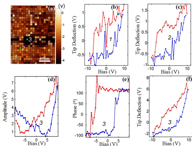
FIG. 2. (Color online) (a) A map of switchable polarization for the \{110\} 1/3\text{PbTiO}_3-2/3\text{CoFe}_2\text{O}_4 film. Dark areas correspond to \text{PbTiO}_3 . (b) and (c) are piezoelectric hysteresis loops at points 1 and 2, respectively. (d) Amplitude of the piezoelectric response at point 3. (e) Phase of the piezoelectric response at point 3. (f) Combined amplitude/phase piezoelectric hysteresis loop at point 3.
