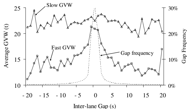
Figure 2. Inter-lane GVW correlation, the Netherlands.
