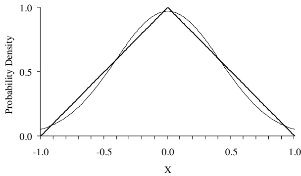
Figure 4. Normal and triangle kernel functions.
