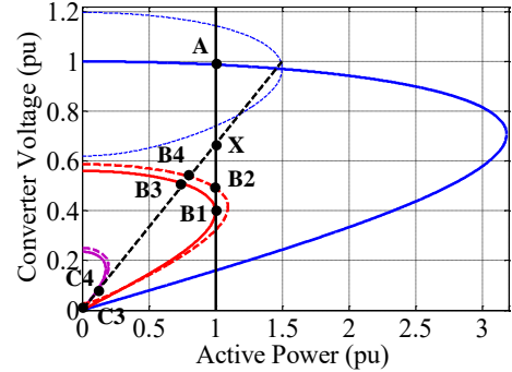
Fig. 2. PV Curve, solid blue line: U_g = 1 pu , dash blue line: U_g = 1 pu, S_{max} = 1.5 pu , solid red line: U_g = 0.56 pu, Q^* = 0 pu , dash red line: U_g = 0.56 pu, Q^* = 0.1 pu , solid purple line: U_g = 0.23 pu, I_{q,max} = 0 pu ; dash purple line: U_g = 0.23 pu, I_{q,max} = -0.1 pu , solid black line: constant power P^* = 1 pu , dash black line: constant current I_{d,max} = 1.5 pu
