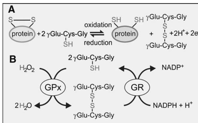
FIG. 4. Oxidation of GSH by (A) non-enzymatic reduction of oxidized protein thiols and (B) GPx-catalyzed reduction of H 2 O 2 . Oxidized GSH is reduced by the NADPH-dependent enzyme, GR. GPx, glutathione peroxidase; GR, glutathione reductase; GSH, glutathione (γ-glutamyl-L-cysteinylglycine); NAD(P)H, nicotinamide adenine dinucleotide phosphate.
