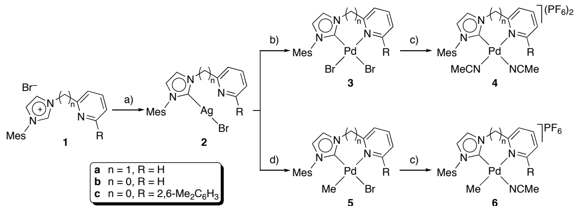
Scheme 1. Synthesis of the complexes (Mes = 2,4,6-Me 3 C 6 H 2 ); reactions and conditions : a) Ag 2 CO 3 , CH 2 Cl 2 , reflux; b) [PdBr 2 (cod)], CH 2 Cl 2 ; c) AgPF 6 , MeCN; d) [PdMeBr(cod)], CH 2 Cl 2 or MeCN.
