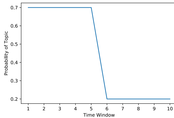
Fig. 1: Example of concept shift, where the probability of a topic appearing changes dramatically over a single time window ( i.e. window 5 to 6).
